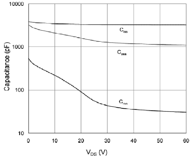
Capacitance
