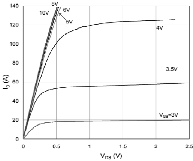
Output Characteristic
